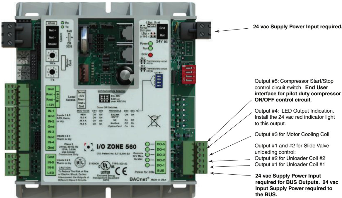
Fig. 22 — Paragon Control Module (PCM)
