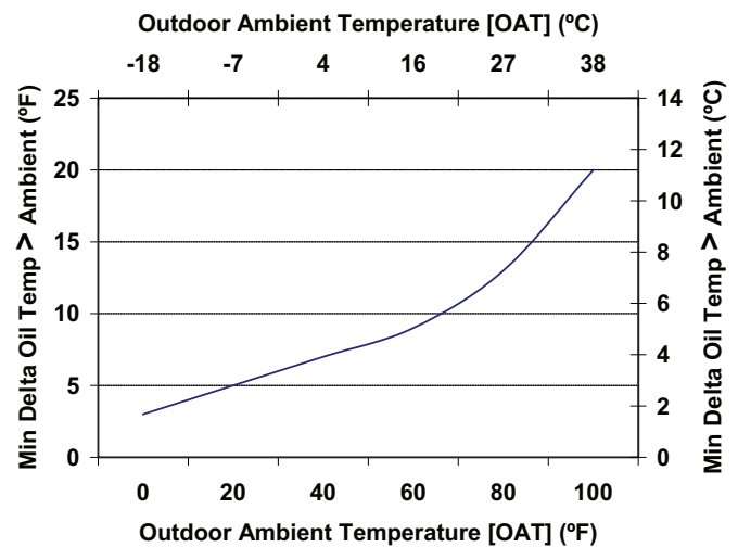
Fig. 7 — Oil Temperature
