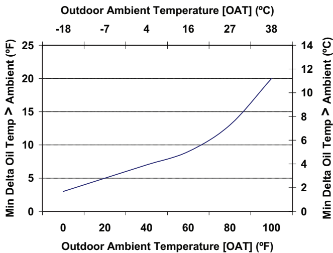
Fig. 12 — Oil Temperature
