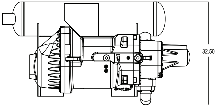
Fig. 35 — 06TSA186 Assembly Drawing
