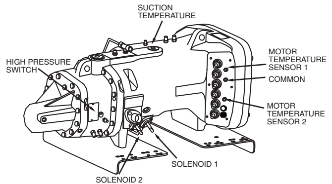
Fig. 13 — Solenoid Locations
