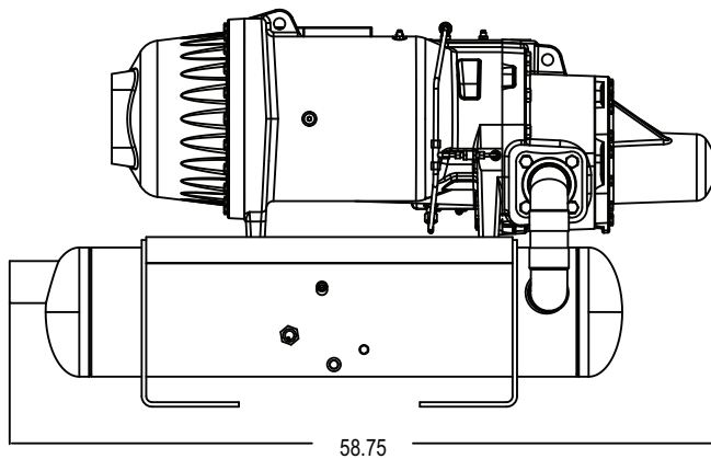
Fig. 36 — 06TTA266 Assembly Drawing
