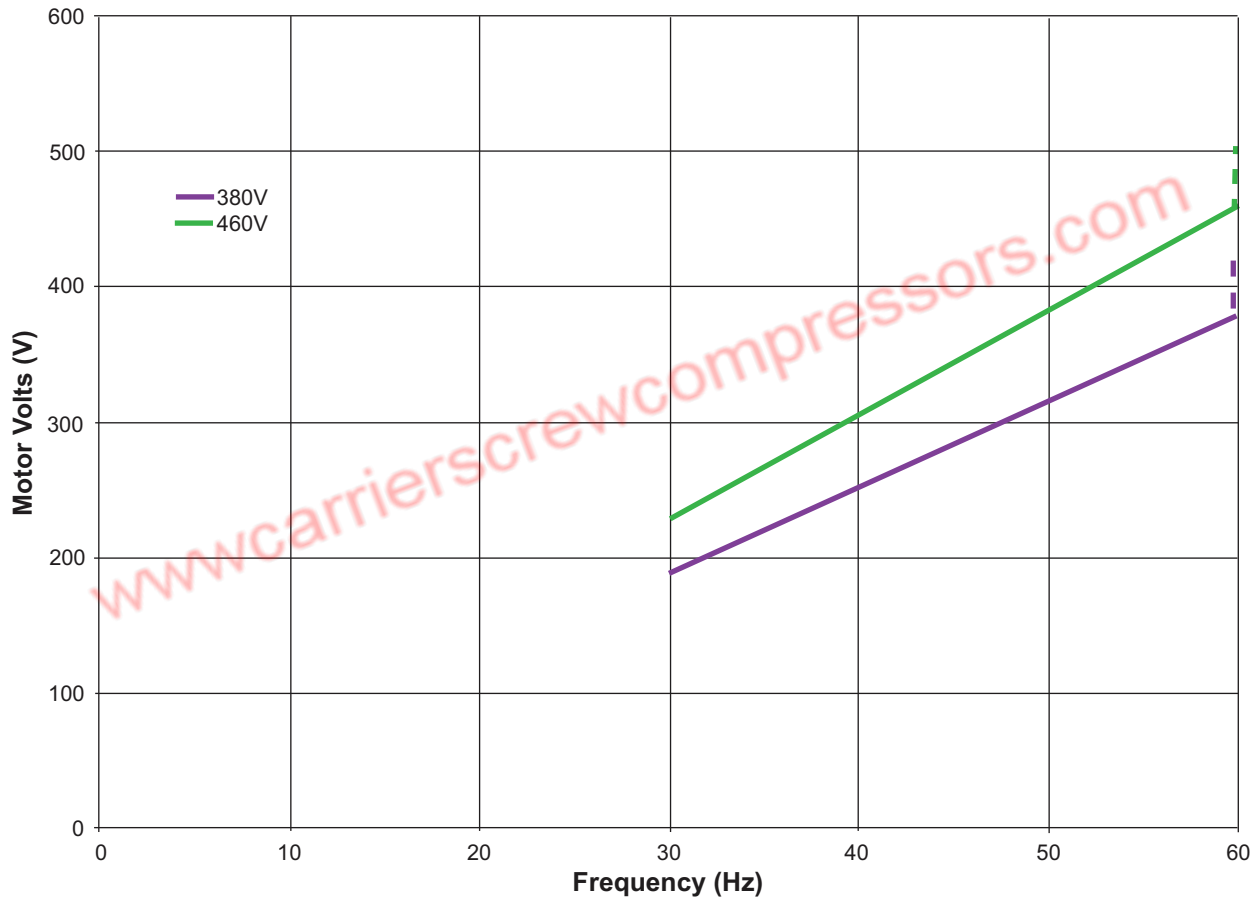
Fig. 28 — Sample Compressor Motor Voltage Curves
