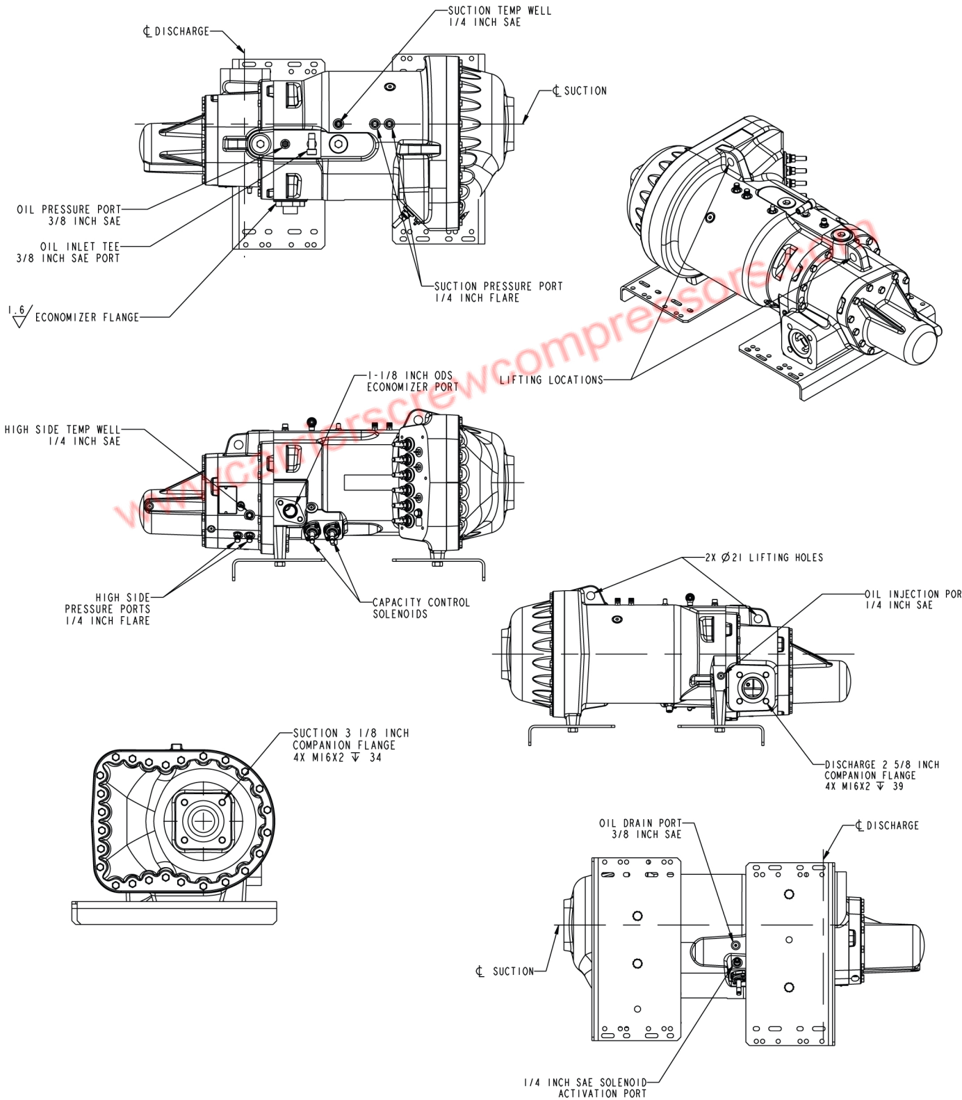
Fig. 1 — 06TS Compressor Physical Data and Connections
