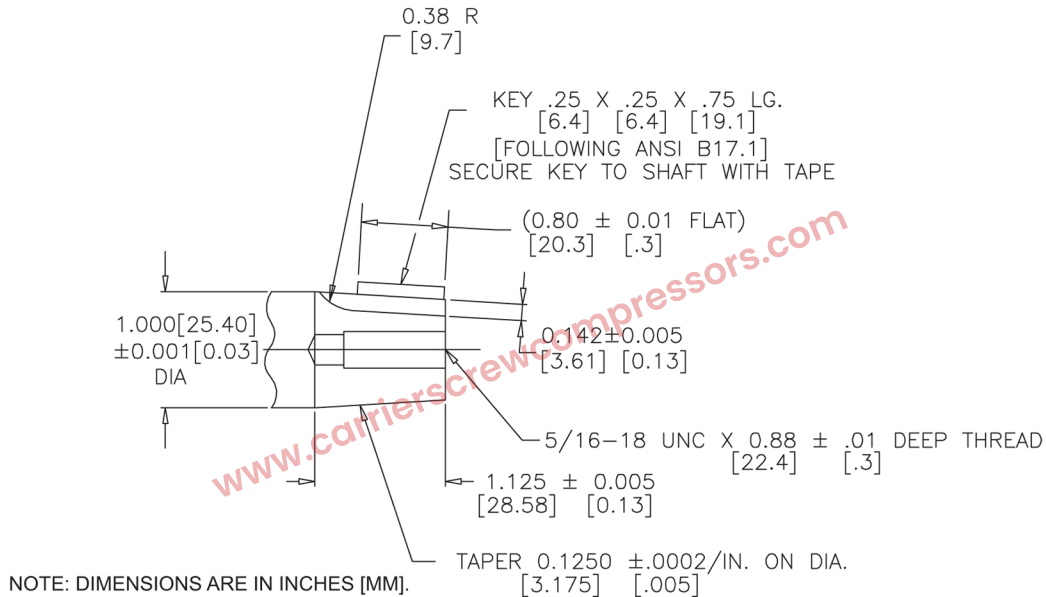
Fig. 11 — 05K 24CFM Shaft Details
